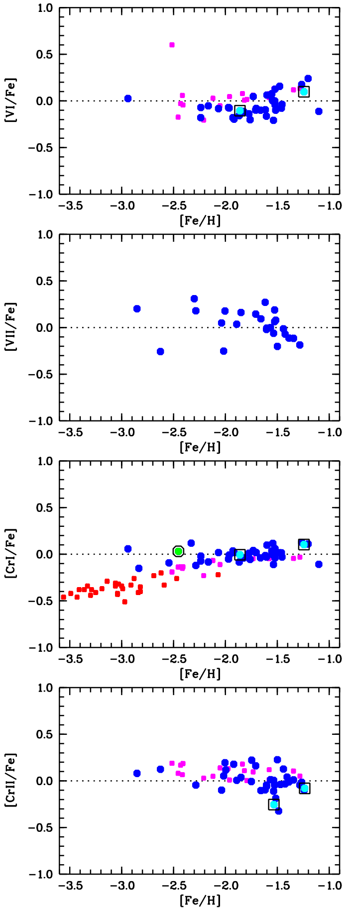
Fig. C.4. [X/Fe] versus [Fe/H] (for V and Cr). Symbols are as in Fig. C.1. In [X/Fe] ratios for the ionised V and Cr, Fe is from Fe II lines.
