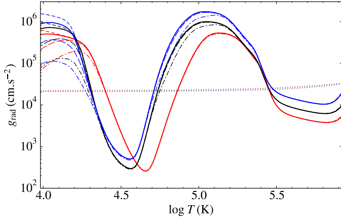
Fig. 1. Radiative accelerations for Sc vs. \log T at the beginning of the MS for a chemically homogeneous 1.5, 1.7, and 2 M_{\odot} model (red, black, and blue sets of curves, respectively). For each mass, the short-dashed, long-dashed, and dash-dotted curves show the g_{\text{rad}} for an abundance one-tenth, ten times, and a hundred times the solar value respectively. The dotted curves denote the local gravity.
