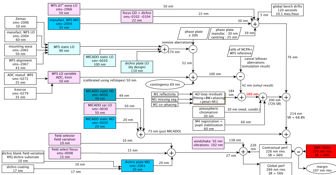
Figure 8. Global SCAO error budget.
