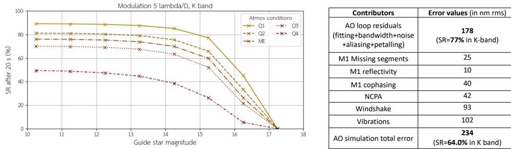
Figure 7. Left: AO simulation based on-axis performance, as a function of reference source magnitude and for different turbulence conditions. Right: SCAO error budget for AO simulation terms, under median atmospheric conditions, at 30° zenith angle, with a 500 Hz loop frequency and a reference source magnitude of 10.
