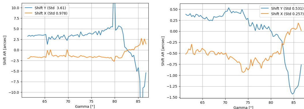
Figure 10. Test results, showing the shifts (X/Y) in position of an image at a given rotation angle (gamma [°]) between the upward and the downward displacements. Left: before design modification (out of spec). Right: after design modification (in spec). Max amplitude during the rotation shall be less than 1.5'' up to gamma \approx 80°.
