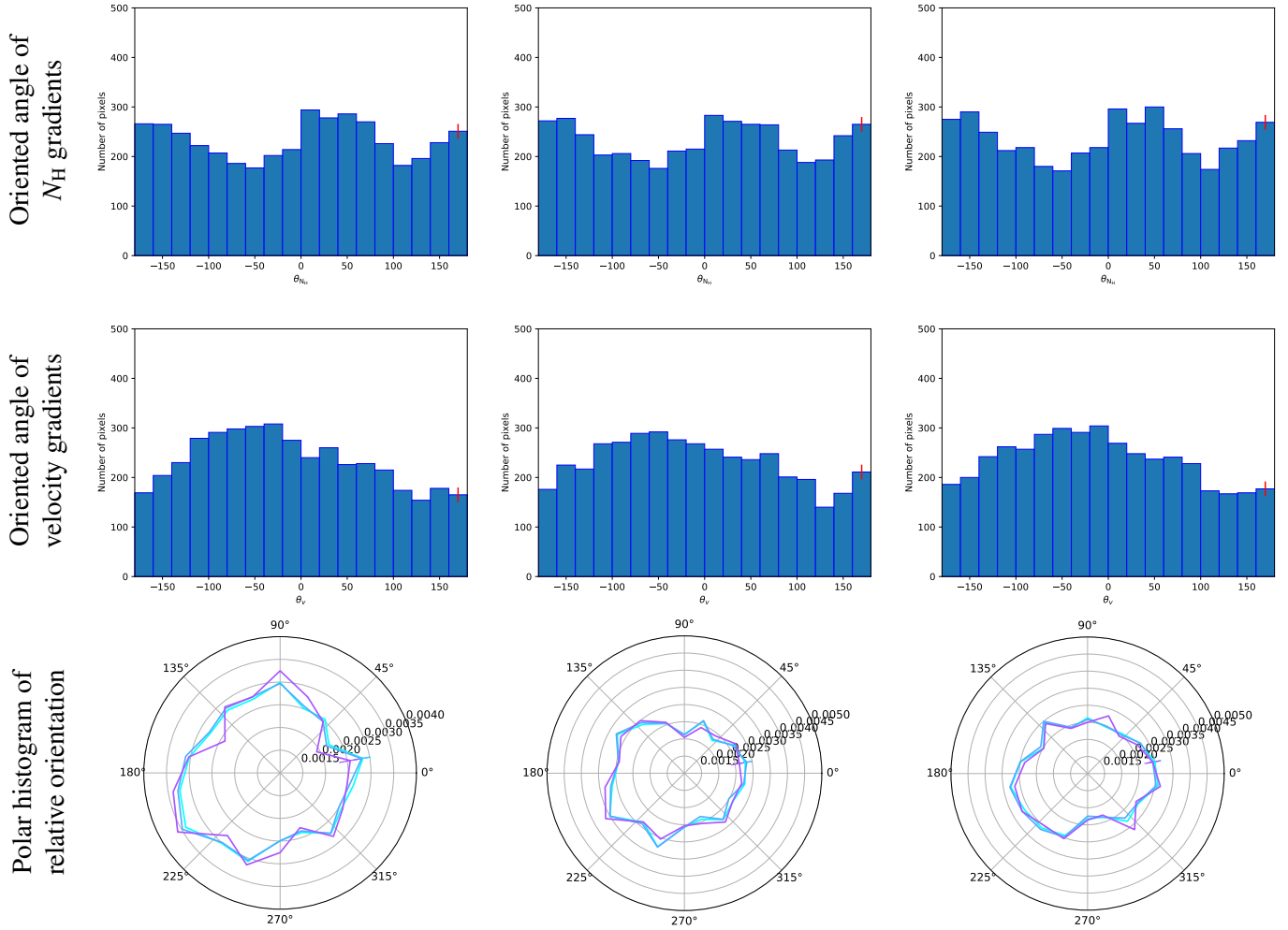
Fig. E.2. \text{C}^{18}\text{O} distribution histogram of the oriented angles of the column density (top row) and velocity gradients (middle row) in the Horsehead nebula from the reference decomposition D0 (left), decomposition D1 (middle) and decomposition D2 (right), respectively. Last row: histograms of the relative orientation between column density and velocity. Data with \log(N_{\text{H}}^{18}) > 21.00 \text{ cm}^{-2} are shown in cyan, \log(N_{\text{H}}^{18}) > 21.55 \text{ cm}^{-2} in blue-violet, \log(N_{\text{H}}^{18}) > 22.00 \text{ cm}^{-2} in purple, and \log(N_{\text{H}}^{18}) > 22.40 \text{ cm}^{-2} in fuchsia. The colored bars at 10^\circ show the error bars of the histograms.
