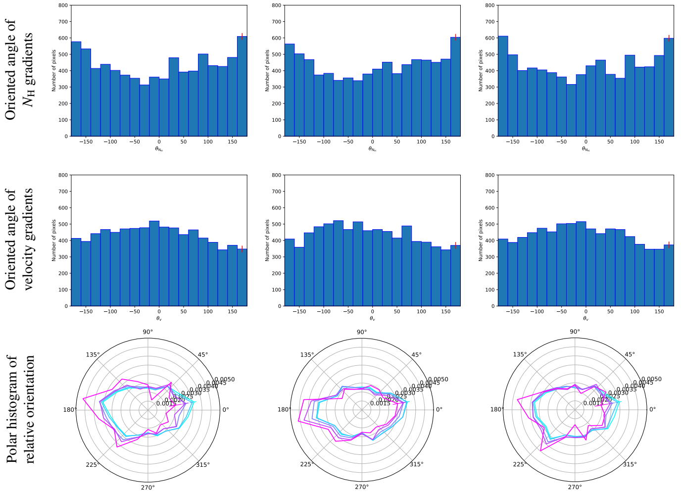
Fig. E.1. ^{13}\text{CO} distribution histogram of the oriented angles of the column density (top row) and velocity gradients (middle row) in the Horsehead nebula from the reference decomposition D0 (left), decomposition D1 (middle) and decomposition D2 (right), respectively. Last row: histograms of the relative orientation between column density and velocity. Data with \log(N_{\text{H}}^{13}) > 20.00 \text{ cm}^{-2} are shown in cyan, \log(N_{\text{H}}^{13}) > 21.00 \text{ cm}^{-2} in blue, \log(N_{\text{H}}^{13}) > 21.55 \text{ cm}^{-2} in blue-violet, \log(N_{\text{H}}^{13}) > 22.00 \text{ cm}^{-2} in purple, and \log(N_{\text{H}}^{13}) > 22.40 \text{ cm}^{-2} in fuchsia. The colored bars at 10^\circ show the error bars of the histograms.
