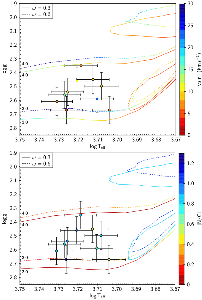
Fig. 11. Log T_{\text{eff}} vs log g diagram for the Georgy et al. (2013) evolutionary tracks with Z = 0.014 , M = 3 M_{\odot} , 4 M_{\odot} , and \omega = 0.3 (solid lines) and 0.6 (dashed lines). Stars in the sample with -0.1 < [\text{Fe}/\text{H}] < 0.1 and M = 3.5 M_{\odot} , 4 M_{\odot} are shown with error bars. Upper panel: Colour index indicates the equatorial velocity for evolutionary tracks and the observed v \sin i for sample stars. Lower panel: Colour index indicates the [\text{N}/\text{C}] abundance ratio.
