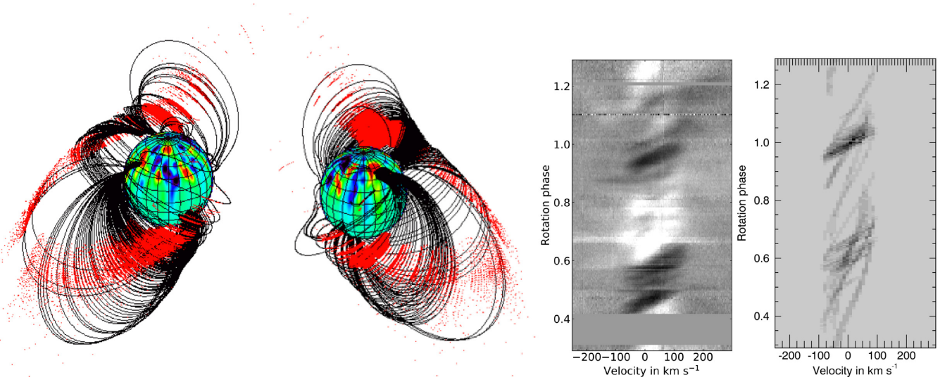
Figure 4. Predicted prominence locations and H\alpha dynamic spectra for AB Dor in Dec 1996. From left to right, panels 1 and 2 show the large-scale field structure with a map of the radial magnetic field painted on the stellar surface (blue denotes negative field, while red is positive). Panel 1 shows phase 0.6, while panel 2 shows phase 1.0. The cool prominence material is shown in red, and samples of the field lines supporting it are drawn in black. The third and fourth panels show the corresponding observed and synthetic H\alpha dynamic spectra, respectively.
