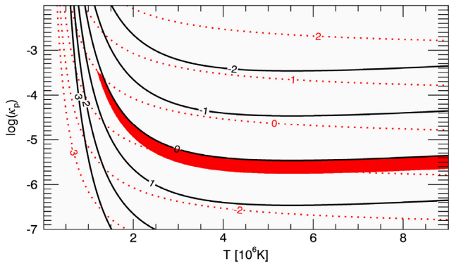
Figure 8. Contours of the logarithms of the prominence lifetimes (black, solid) and plasma \beta at the coronation radius (red, dotted) for a range of value of the free parameters \kappa_p and loop temperature T . Within the red shaded region, the prominence lifetimes lie in the range 1 < \tau[\text{d}] < 10 and the plasma \beta < 1 .
