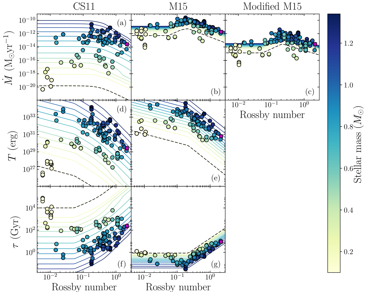
Figure 3. : Mass-loss rate (top), angular momentum-loss rate (middle) and spin-down time-scale (bottom) as a function of Rossby number. These quantities are calculated using (or are associated with) the CS11 (left), M15 (center) and modified M15 (right) models. Each point is colour coded by stellar mass. Solid lines correspond to the parameter of interest in each panel calculated for a given stellar mass over a range of Rossby numbers (see text for details). The solid lines are plotted in intervals of 0.1M_{\odot} from 0.1M_{\odot} to 1.3M_{\odot} and are also colour coded by stellar mass. The lines corresponding to 0.1M_{\odot} have been plotted with a dashed black line for visibility. The average solar value in each panel is shown with a magenta square and the range of variability is shown with a magenta strut when applicable.
