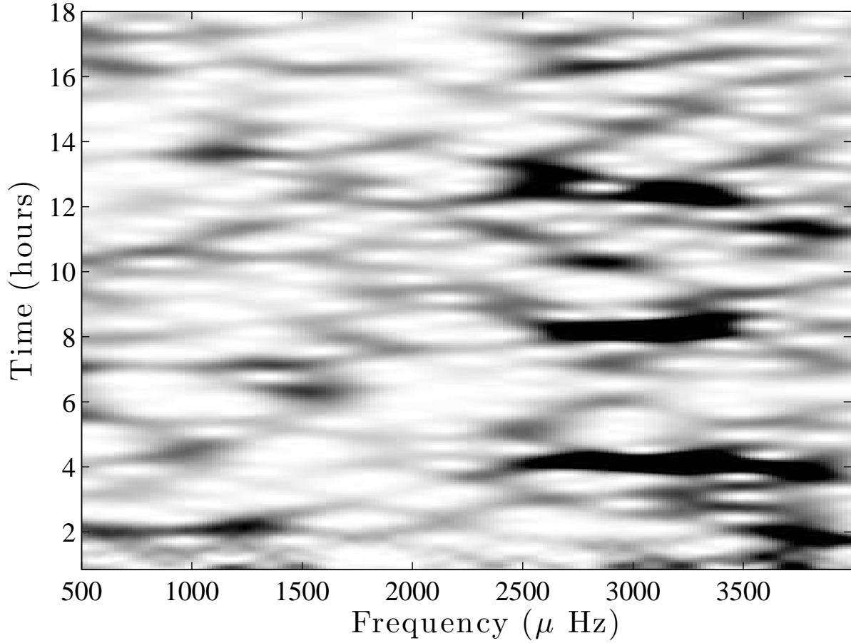
Figure 5. Envelope of the autocorrelation function (EACF) as function of frequency ( x -axis) and time ( y -axis). The EACF was computed every 20 \mu\text{Hz} from 500 to 4000 \mu\text{Hz} , by filtering the time-series in a frequency bandpass of 500 \mu\text{Hz} . The darker a region is, the larger the correlation. Solar modes are clearly visible in between 2500 and 3500 \mu\text{Hz} at approximately 4 , 8 and 13 hours.
