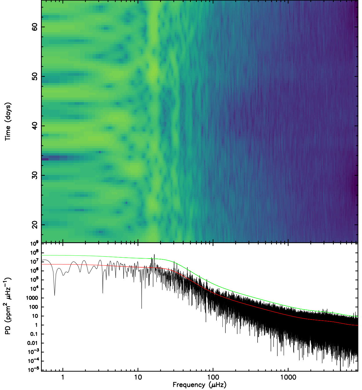
Figure 4. The bottom panel plots the power spectral density (PSD) of the distance corrected photometry. The calculation is described in §4. The red line shows the fitted PSD model based on Equation 8 which is an estimate of the mean. The green line is 9.89 times the PSD model and presents our adopted cut to identify significant frequencies as described in §4.1. The top panel shows a windowed PSD to demonstrate variability in PSD as a function of time. Light, green colour represent larger values of the PSD and darker bluer colours correspond to lower values of the PSD.
