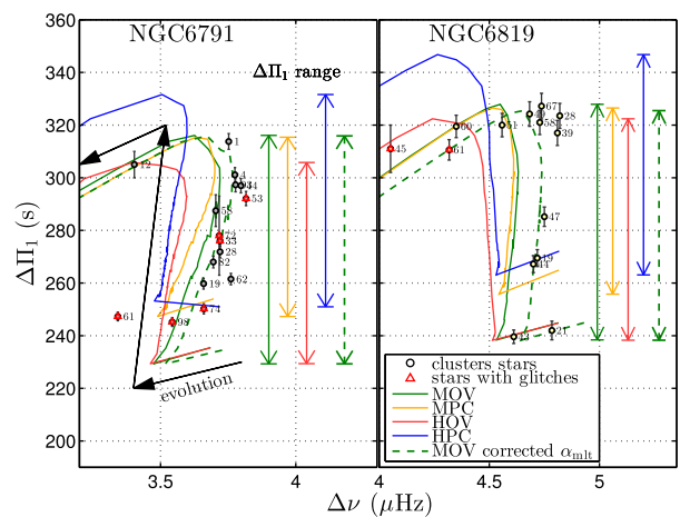
Figure 1. RC stars in NGC 6791 and NGC 6819 in a \Delta\Pi_1 – \Delta\nu diagram. Model predictions based on different near-core-mixing schemes are shown by solid lines. The vertical lines indicate the range of \Delta\Pi_1 covered by each mixing scheme. The dashed line shows MOV models computed with slightly ( \lesssim 3 per cent) increased mixing-length parameters (compared to the solar-calibrated value). The red triangles mark the presence of buoyancy glitches that, to the first order, induce a modulation in \Delta\Pi_1 with respect to the asymptotic value (Miglio et al. 2008; Cunha et al. 2015, and fig. 10 of Mosser et al. 2015), potentially hampering an accurate inference of the asymptotic \Delta\Pi_1 .
